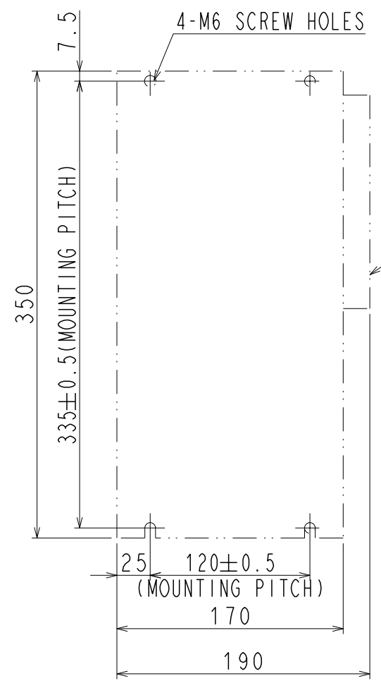
MOUNTING HOLE DIAGRAM
