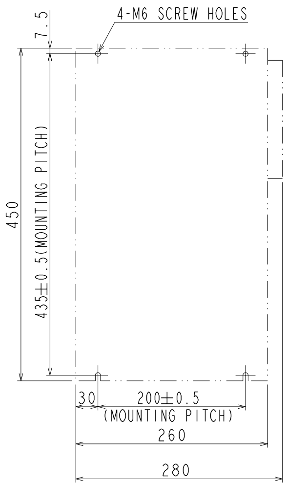
MOUNTING HOLE DIAGRAM
