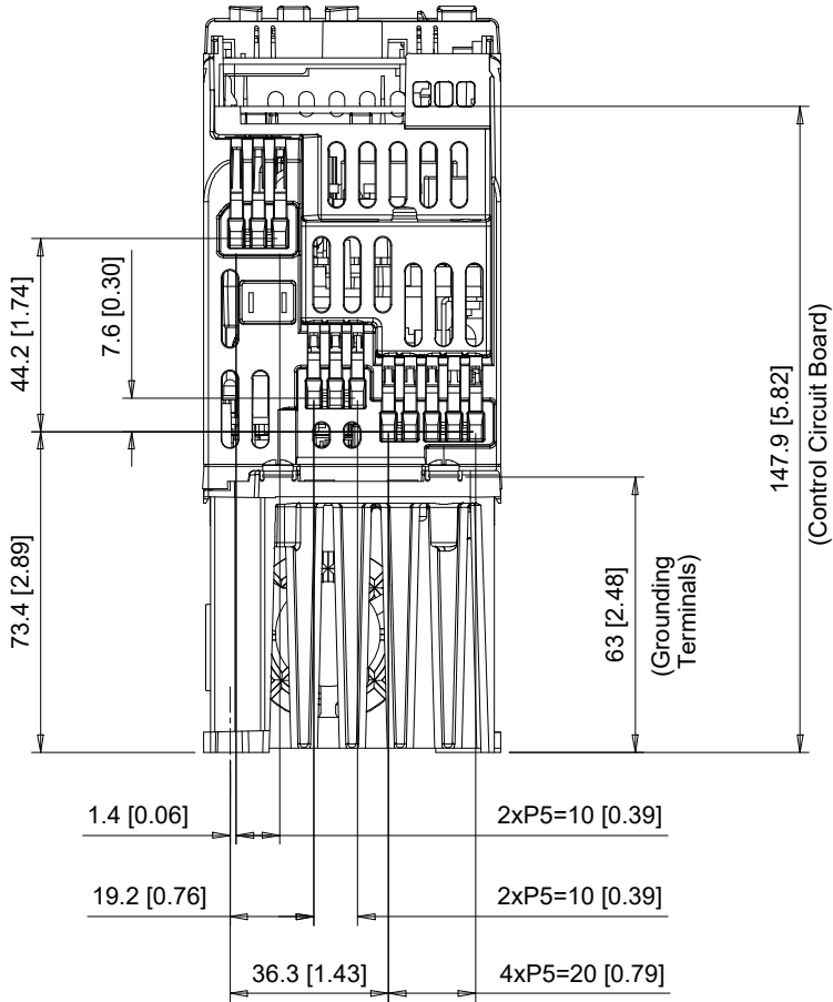
BOTTOM VIEW
