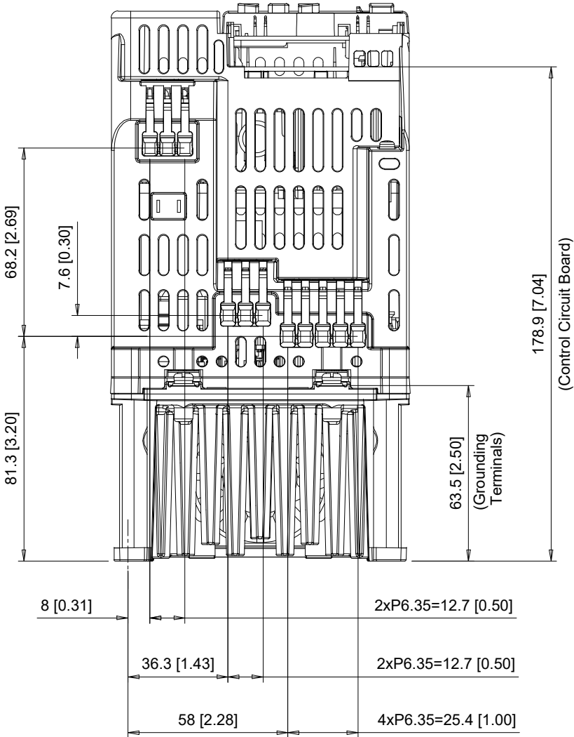
BOTTOM VIEW
