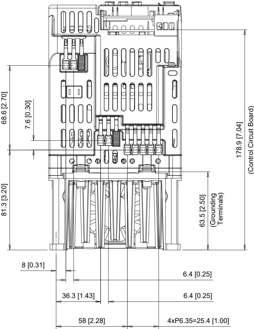
BOTTOM VIEW
