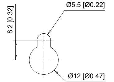
Detail A Top mounting hole dimensions Scale 1:1
