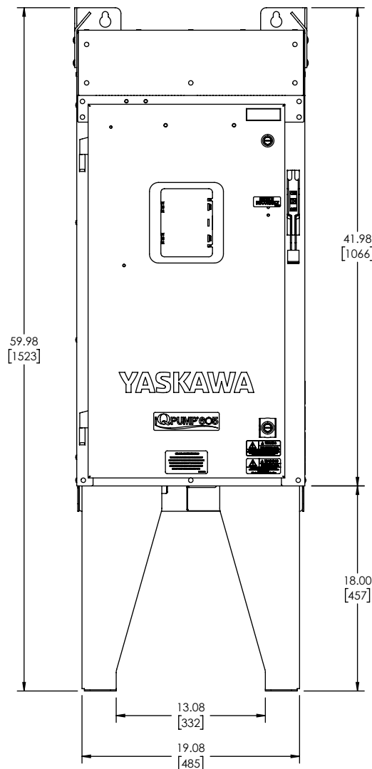
18" HIGH LEGS
