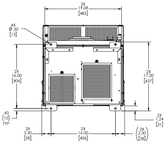
18" HIGH LEGS
