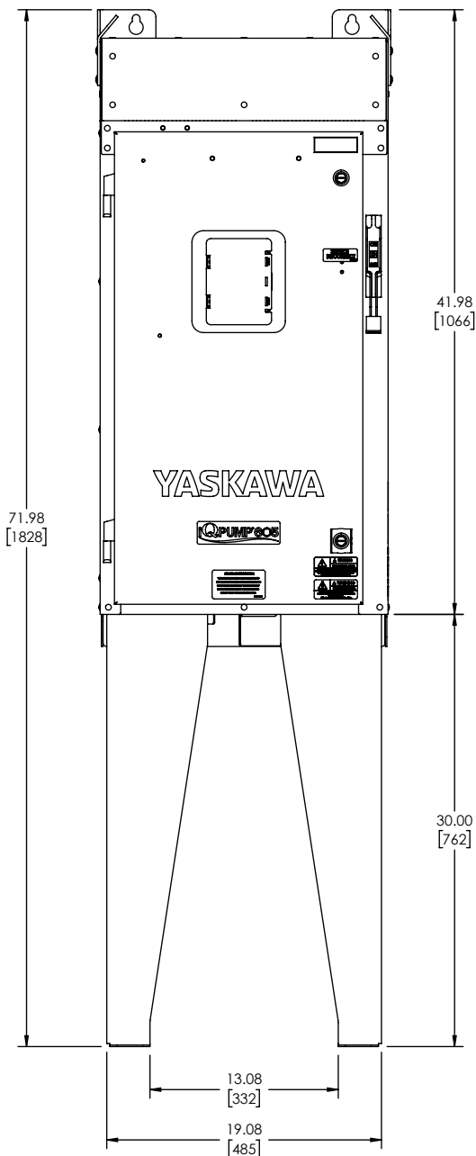
30" HIGH LEGS
