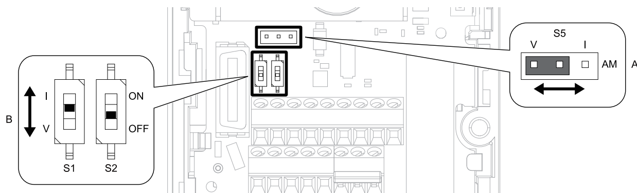
Figure 9 HV305 Switches and Jumpers
