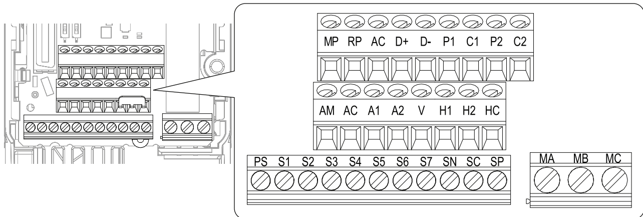
Figure 5 HV305 Control Circuit Terminals
