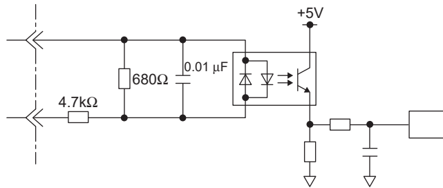
Input Circuit
