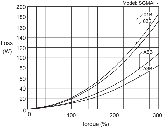
SGMAH Servomotors
