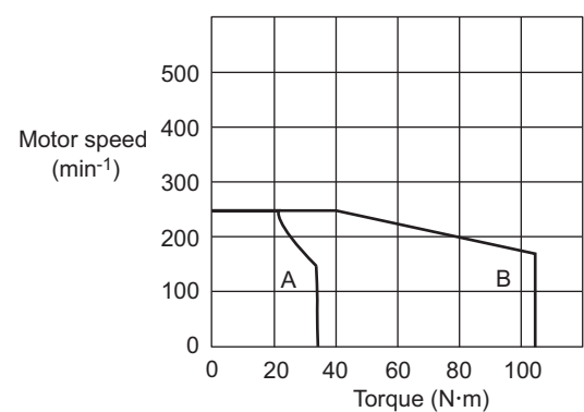
SGMCS-35E□B
