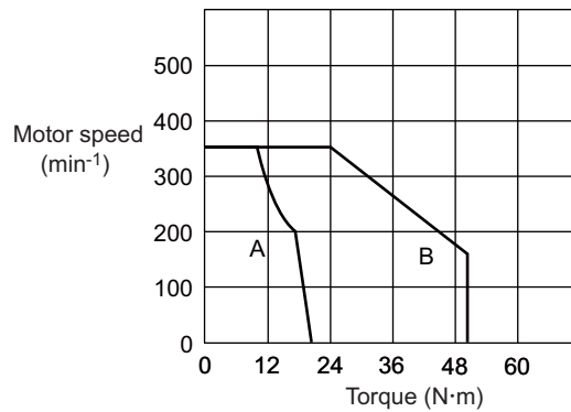
SGMCS-17D□C
