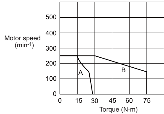
SGMCS-25D□C
