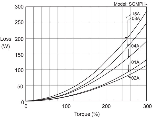
SGMPH Servomotors
