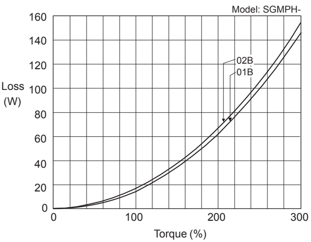
SGMPH Servomotors
