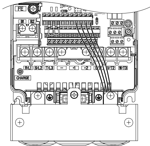
Figure i.14 Terminal Board Location Inside the Drive
