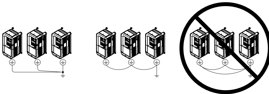
Figure i.10 Multiple Drive Wiring
