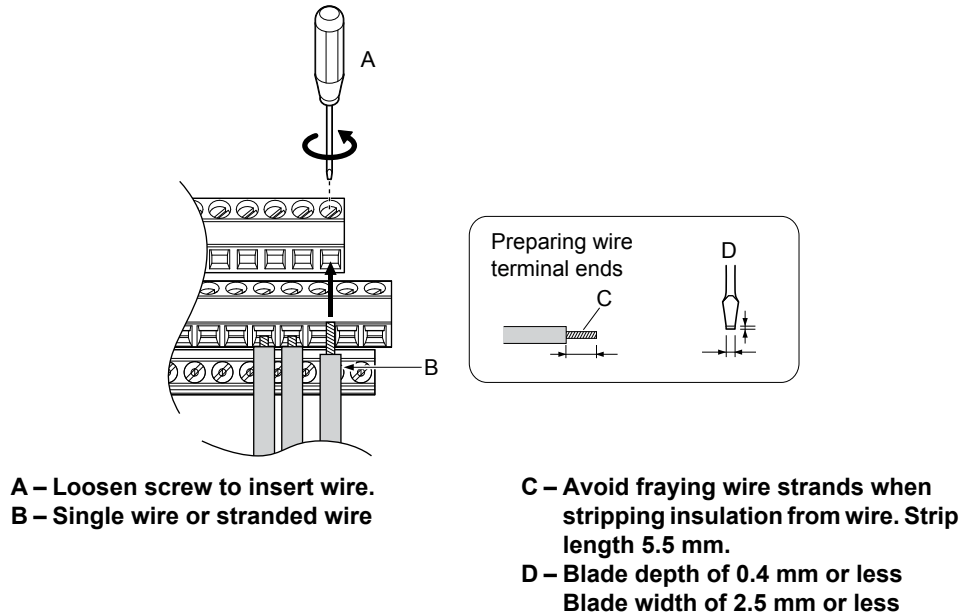
Figure i.13 Terminal Board Wiring Guide
