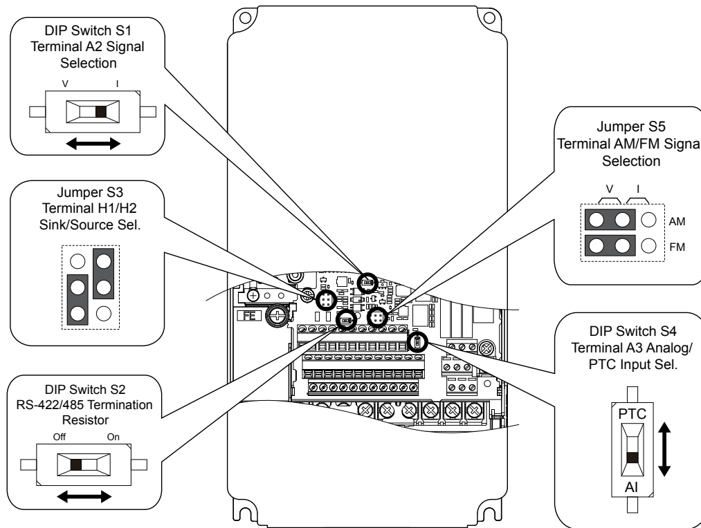
Figure i.16 Locations of Jumpers and Switches on the Terminal Board
