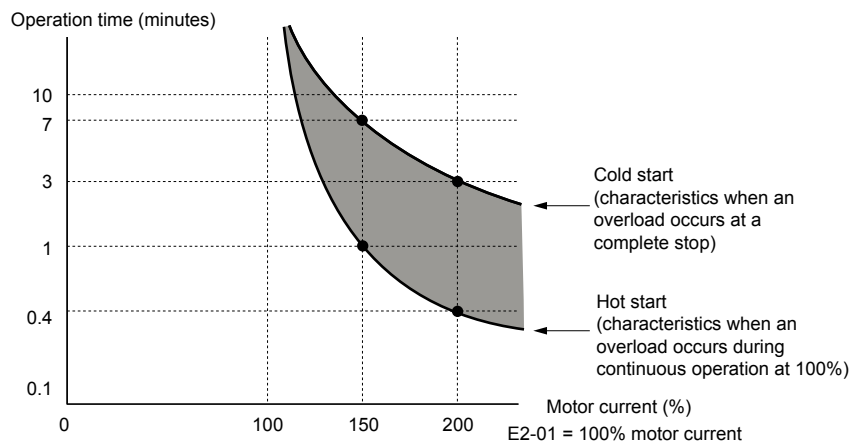
Figure i.20 Motor Overload Protection Time
