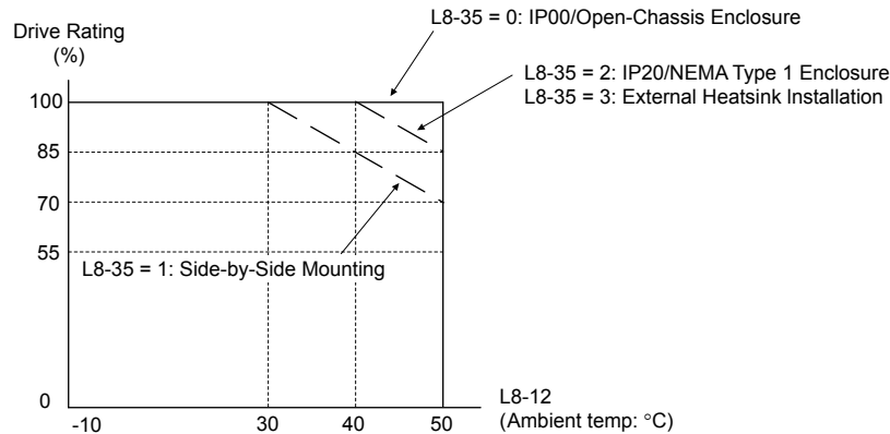
Figure i.22 Ambient Temperature and Installation Method Derating
