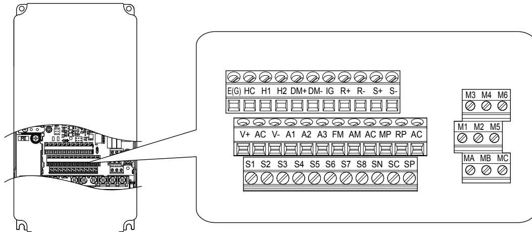
Figure i.11 Control Circuit Terminal Arrangement
