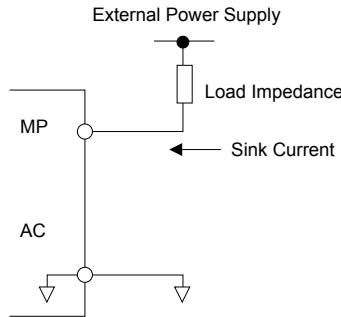
Figure i.17 Pulse Output Connection Using External Voltage Supply
