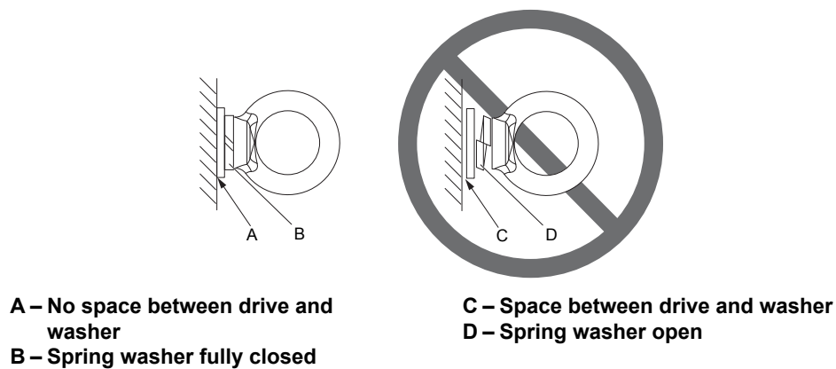
Figure i.1 Spring Washer
