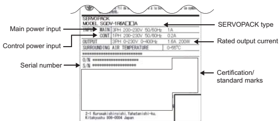
SERVOPACK nameplate
