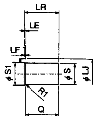
Detailed View of Shaft End
