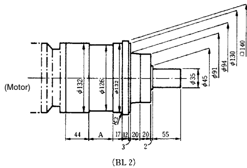
Detailed dimensions of IMT gear
