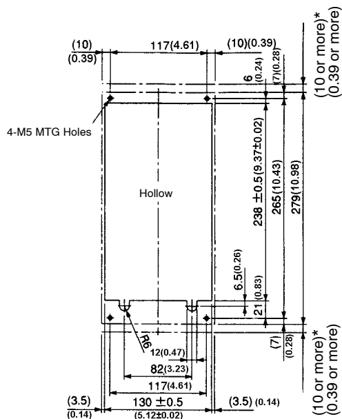
Mounting Surface Diagram
