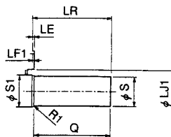
Detailed View of Shaft End for SGMG-1AASAAB and -1EASAAB
