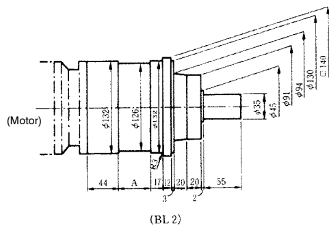
Detailed dimensions of IMT gear
