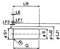
Detailed View of Shaft End for SGMG-1AA2AAB and -1EA2AAB
