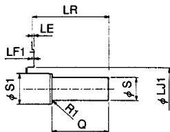
Detailed View of Shaft End for SGMG-05ASAAB to -13ASAAB
