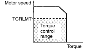
Speed Control Range for Torque Control
