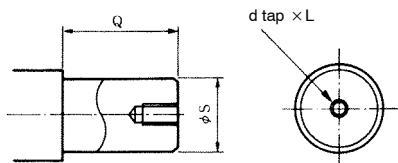
Shaft end tap specifications
