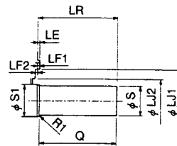
Detailed View of Shaft End for SGMG-55ASAAB and -75ASAAB
