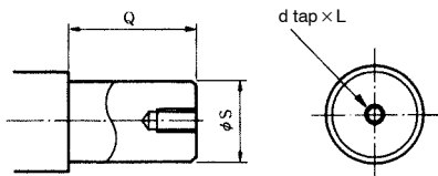
Shaft end tap specifications
