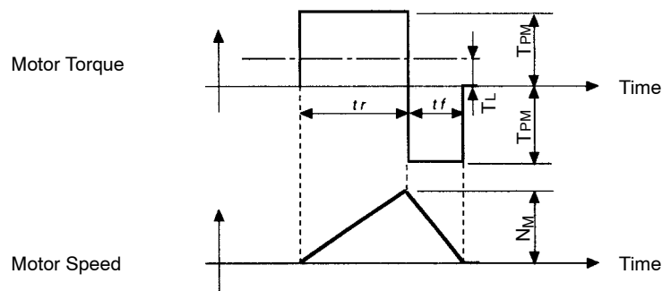
Motor Torque (size) - Motor Speed Timing Chart
