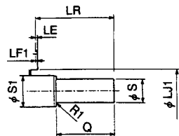
Detailed View of Shaft End for SGMG-05A2AAB to -13A2AAB
