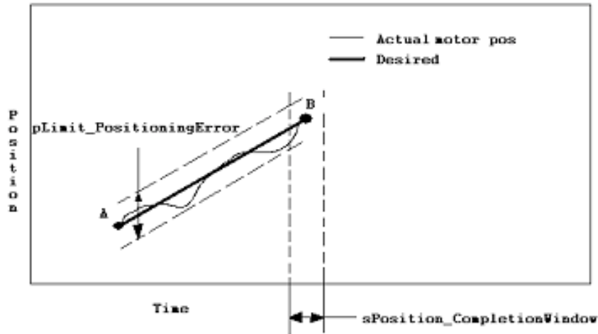
A simple move profile from A to B
