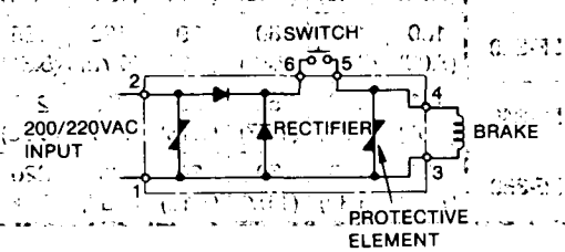
Type OPR109A Circuit Diagram
