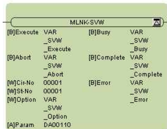
Figure 4. MECHATROLINK Servo Write instruction
